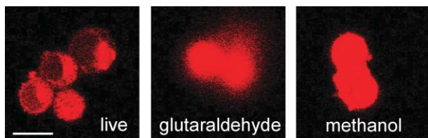
Fig. 4 The cells were incubated in presence of 500 \mu\text{M} of the helicite in RPMI-1640 for 24 h. The images were taken as for Fig. 2. Scale bar: 17 \mu\text{m} .
